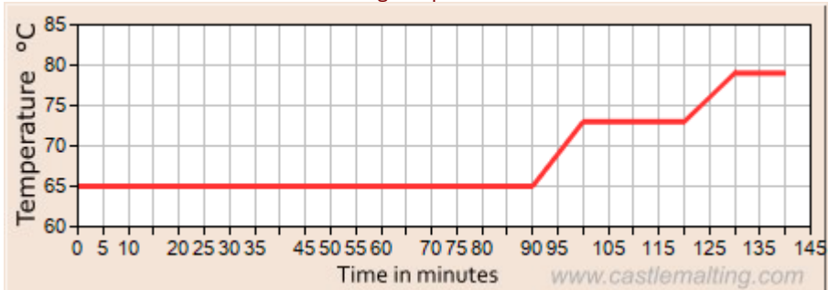
Mashing temperature
